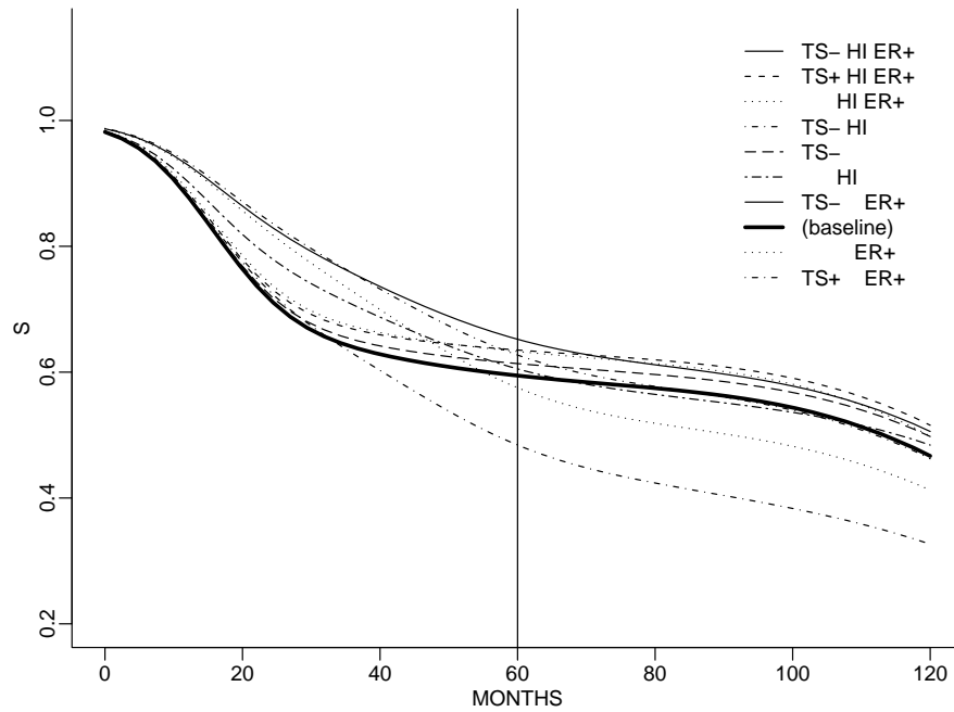
Figure 4: Survival example: Posterior predictive survival function S(t | x) \equiv p(y_{n+1} > t | x_{n+1} = x, \text{data}) , arranged by x . The “baseline” case refers to all continuous and count covariates equal to the empirical mean, and all binary covariates equal 0. The legend indicates TS- and TS+ for tumor size equal 26mm and 50mm (first and third empirical quartile), HI for HI = 1 and ER+ for ER = 1. The legend is sorted by the survival probability at 5 years, indicated by a thin vertical line.
