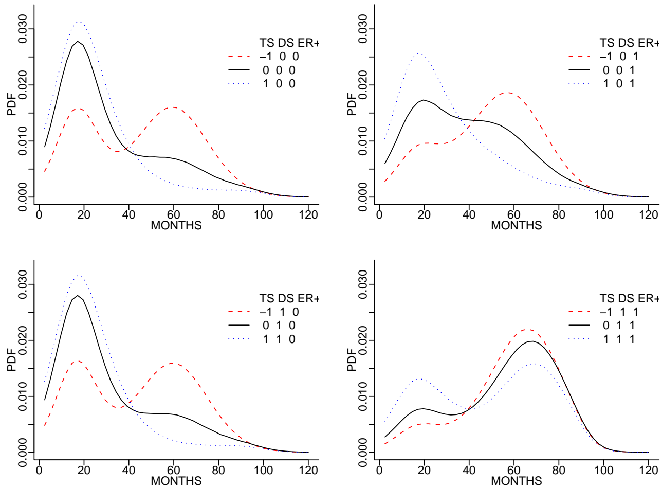
Figure 1: Simulation truth p.d.f. for the outcome variable for different combinations of the three covariates.
