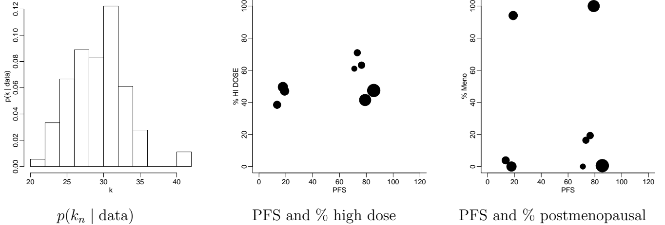
Figure 5: Survival example: Posterior distribution for the number of clusters (left panel), mean PFS and % high dose patients per cluster (center panel), mean PFS and % postmenopausal patients per cluster (right panel).
