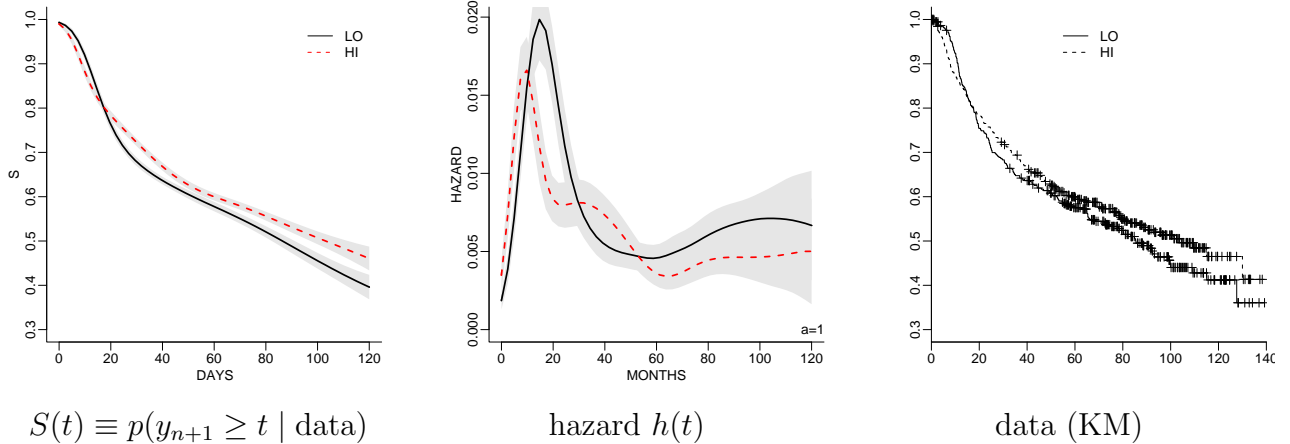
Figure 2: Survival example: Estimated survival function (left panel) and hazard (center panel), arranged by x \in \{HI, LO\} . The grey shades show point-wise one posterior predictive standard deviation uncertainty. The right panel shows the data for comparison (Kaplan-Meier curve by dose).
