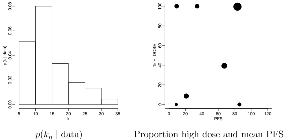
Figure 3: Survival example: Posterior for the number of clusters k_n (left panel), and proportion of patients with high dose (%HI) and average progression free survival (PFS) by cluster. The size (area) of the bullets is proportional to the average cluster size.
